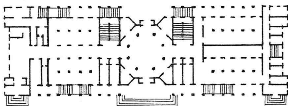
Figure 13. Pyongyang Station, 1st Floor Plan (source: Korean Architecture , 1989, No. 2)
